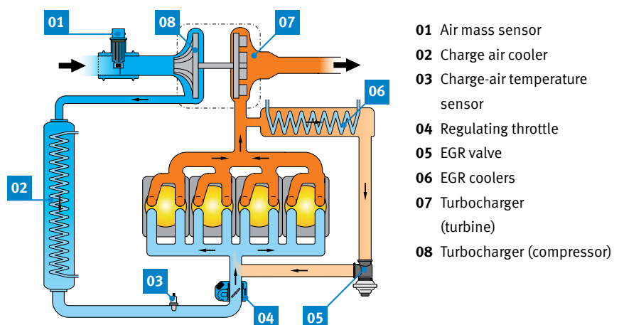
Fig. 2: Schematic diagram of cooled exhaust gas recirculation
